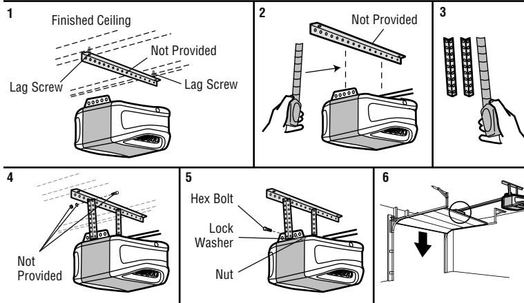
Finished Ceiling
